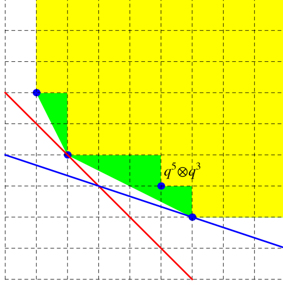
Figure 1. Typical element E \in \text{Sub}_{\ge}(\mathbb{N} \times \mathbb{N}) (in yellow); its image under \mu (red), under the Frobenius correspondence for \lambda = \frac{1}{3} (blue) and under \gamma (green or yellow). Removing the element q^5 \otimes q^3 does not alter the convex hull \gamma(E) .
