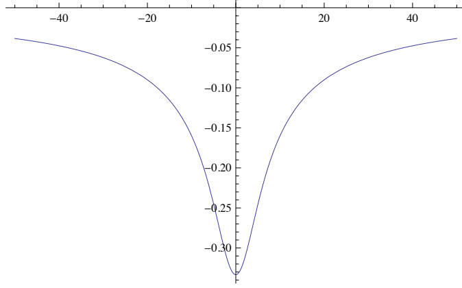
FIGURE 6. Graph of the function K_2 - \frac{1}{3} , even and negative.
