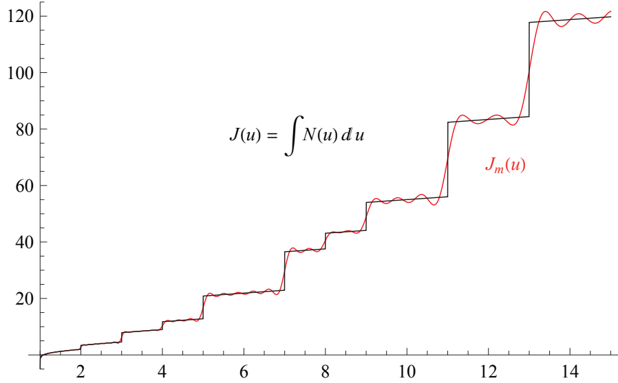
FIGURE 1. Primitive J(u) of N(u) and approximation using the symmetric set Z_m of first 2m zeros, by
